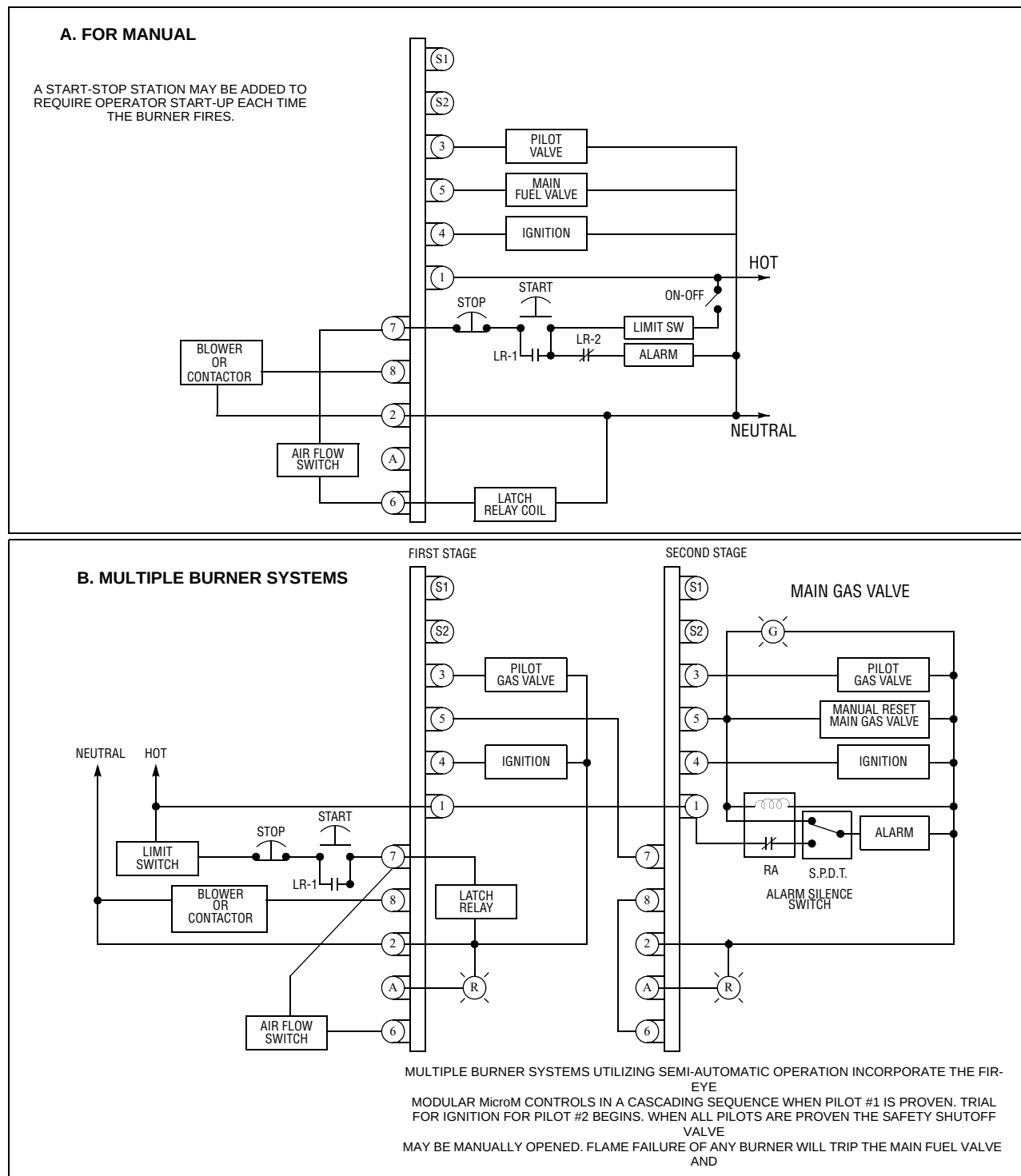
FIGURE 13. ALTERNATE WIRING ARRANGMENT FOR MEP CONTROLS
