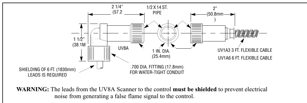
FIGURE 17. UV8A Scanner
