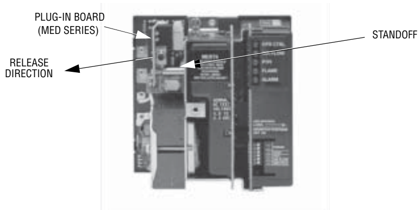
FIGURE 4. PLUG-IN BOARD LOCATION AND INSTALLATION
