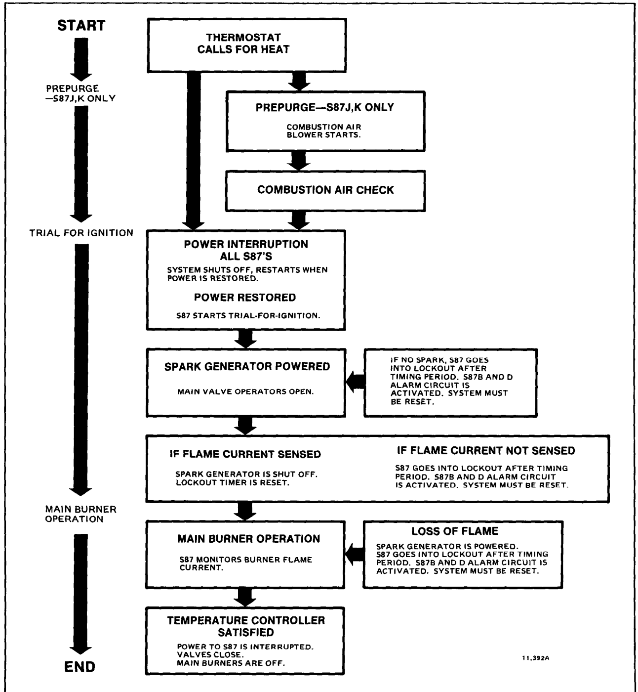
FIG. 10—NORMAL SYSTEM SEQUENCE OF OPERATION.
