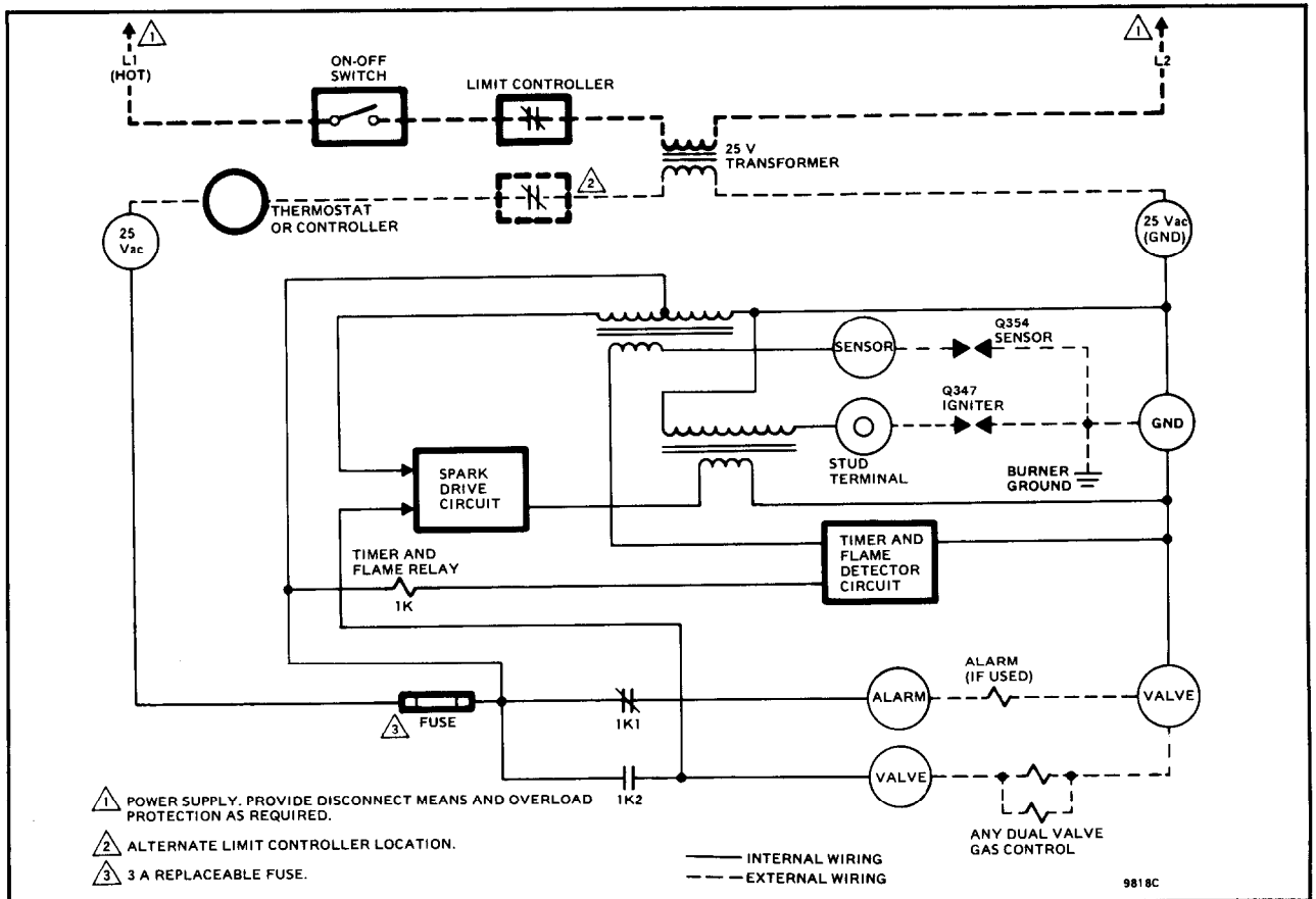
FIG. 16—S87D SIMPLIFIED SYSTEM SCHEMATIC.
