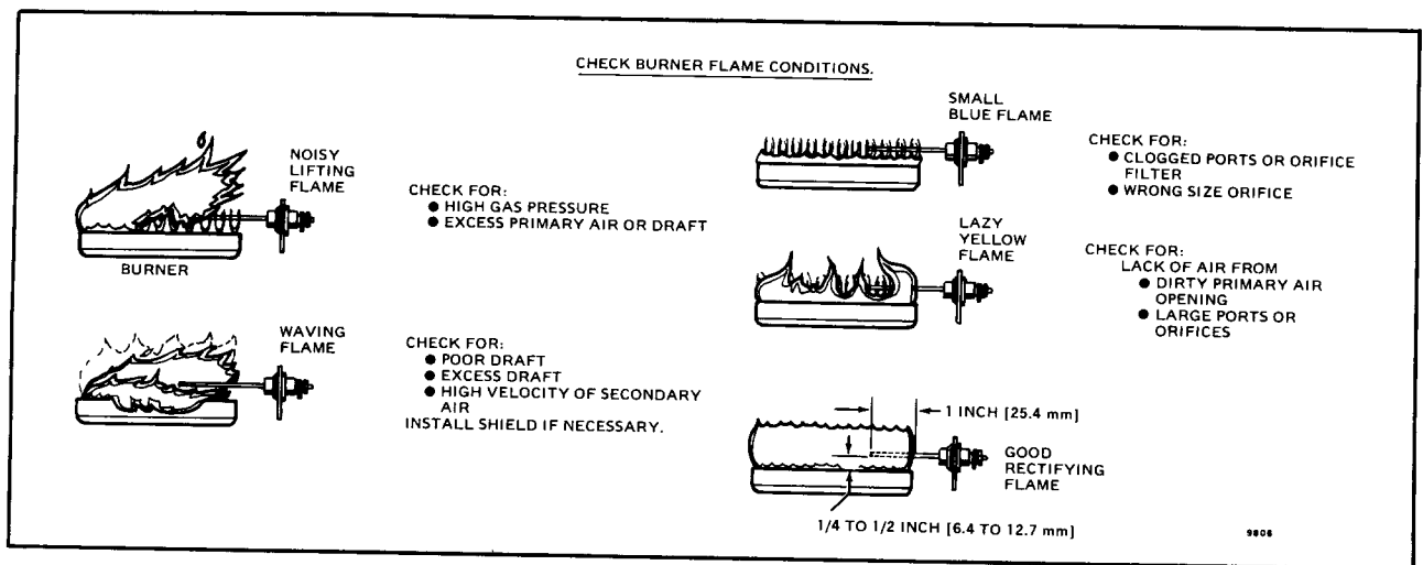
FIG. 12—CHECK BURNER FLAME CONDITIONS.
