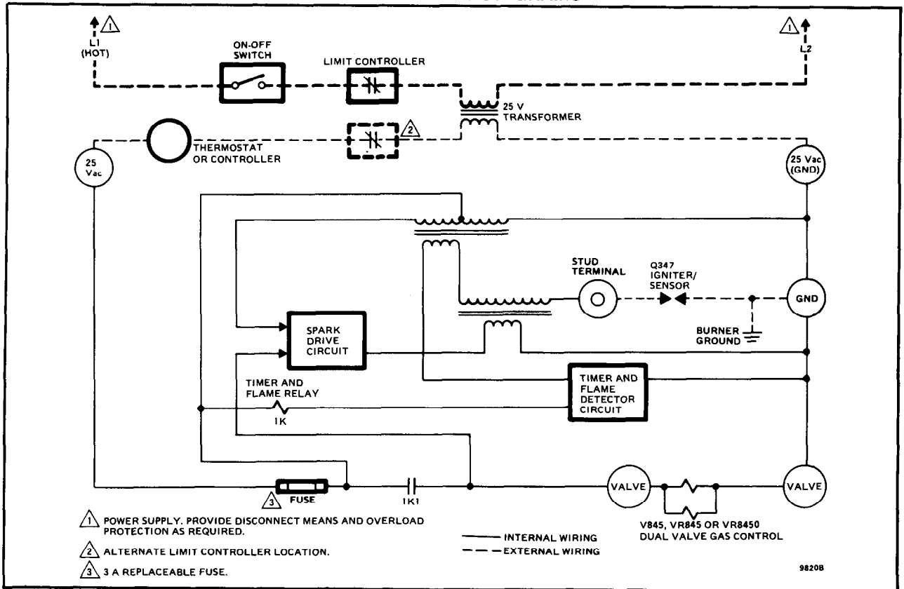
FIG 13—S87A SIMPLIFIED SYSTEM SCHEMATIC.
