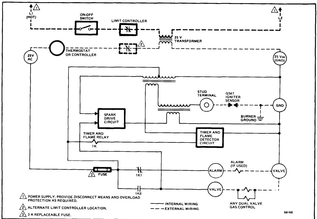
FIG. 14—S87B SIMPLIFIED SYSTEM SCHEMATIC.
