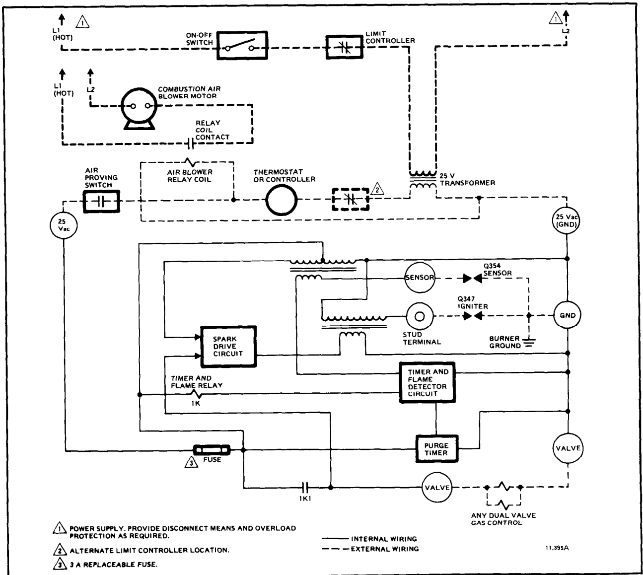
FIG. 18—S87K SIMPLIFIED SYSTEM SCHEMATIC.
