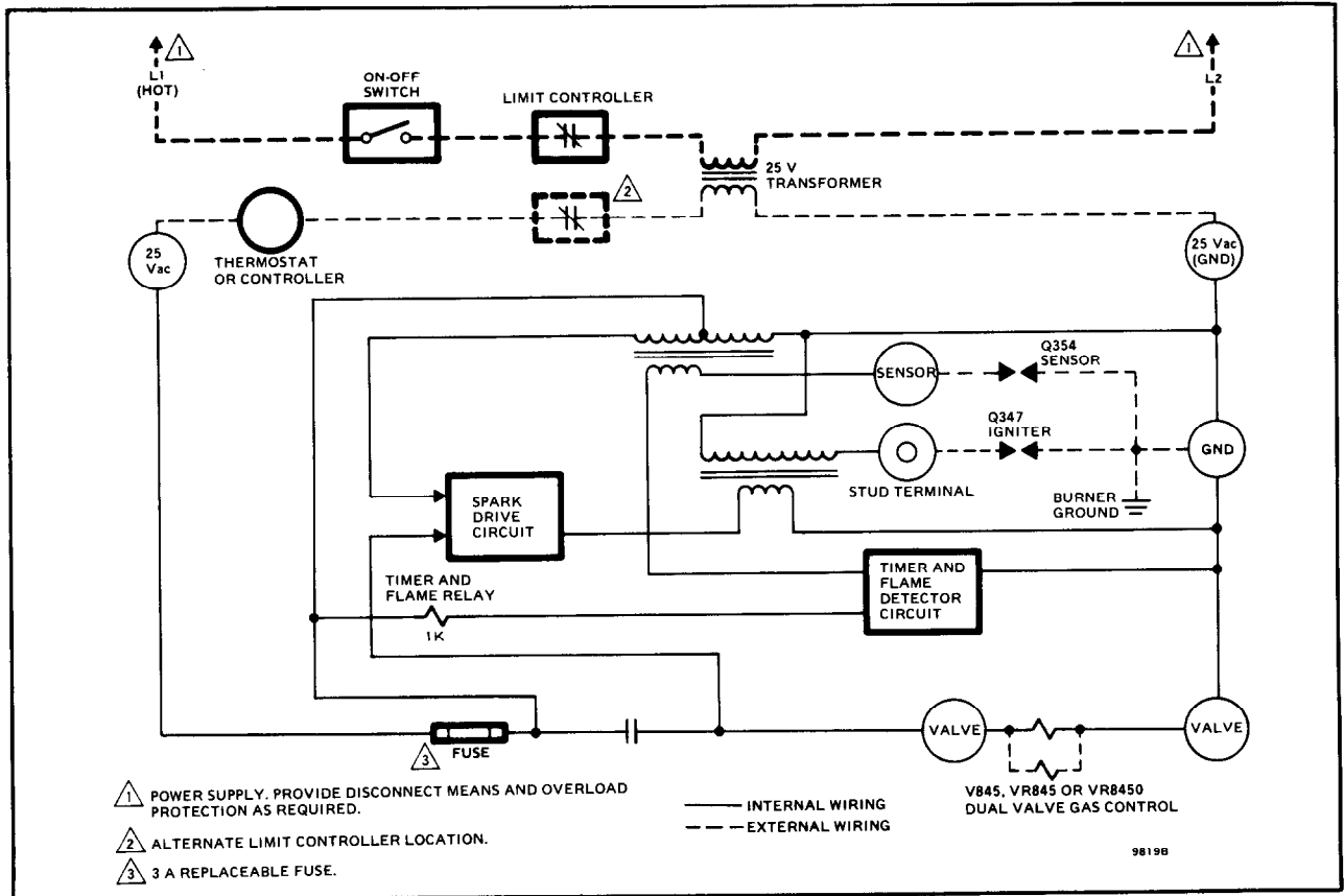
FIG. 15—S87C SIMPLIFIED SYSTEM SCHEMATIC.
