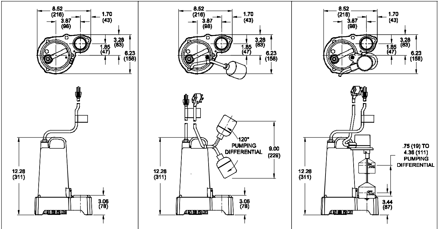
Model: SP75AX Mech. Wide Angle Float
