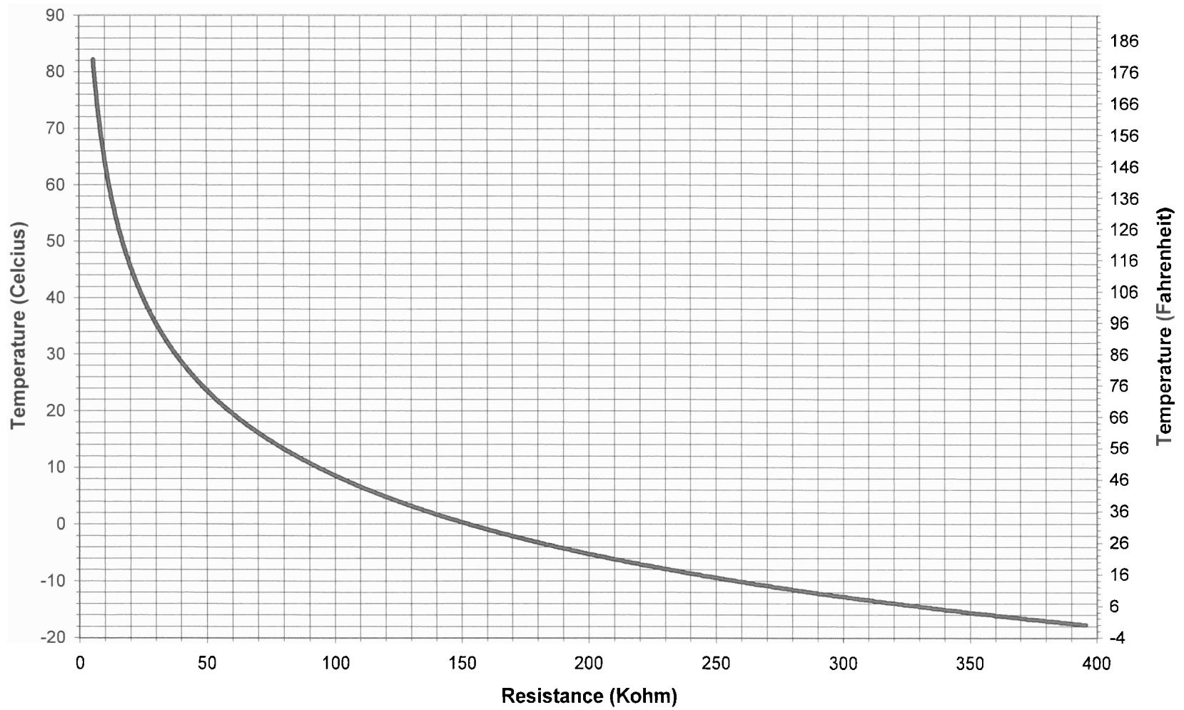
Resistance Chart for 47Kohm Temperature Sensor
